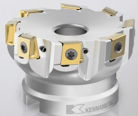
Mill 4™-12 KT
